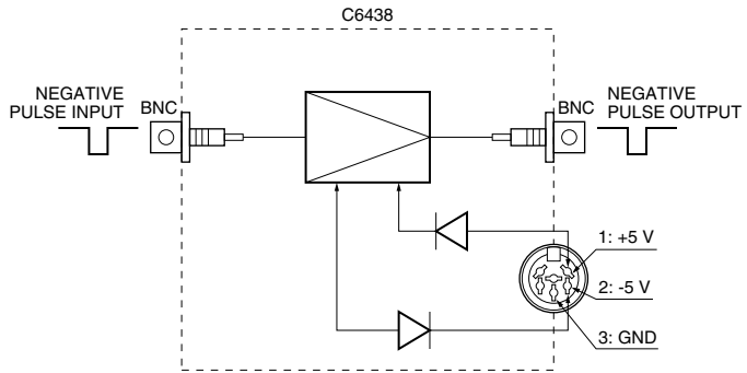
Figure 3: Internal Connection Diagram
